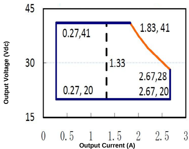
Figure 1: Typical V-I Characteristic Curve (LUB075X-041C)
