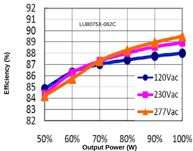
Figure 5: Efficiency vs. Output Power ( I_o=1.88A )
