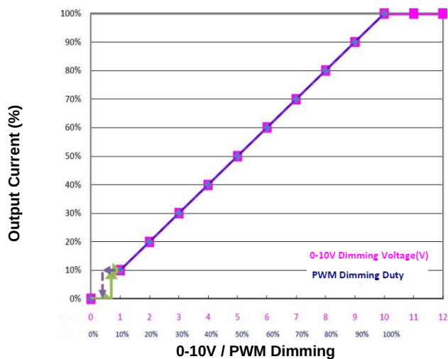
Figure 13: 0-10V/PWM Dimming Curve
