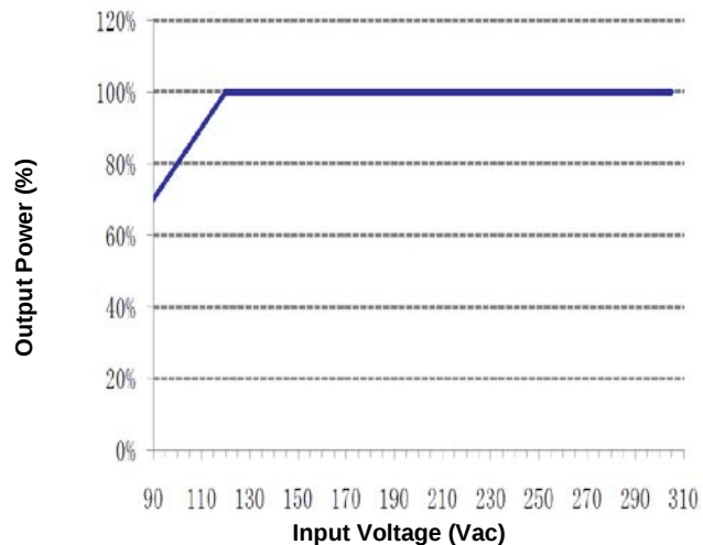
Figure 9: Output Power vs. Input Voltage
