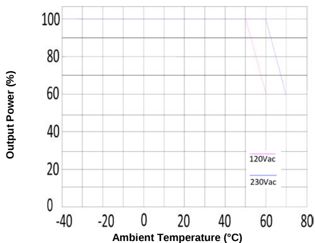
Figure 8: Output Power vs. Ambient Temperature
