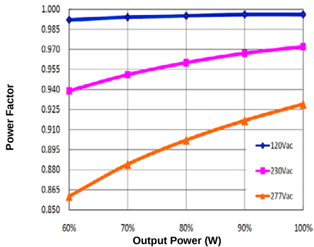
Figure 11: Power Factor vs. Output Power
