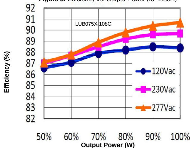
Figure 7: Efficiency vs. Output Power ( I_o=1.05A )
