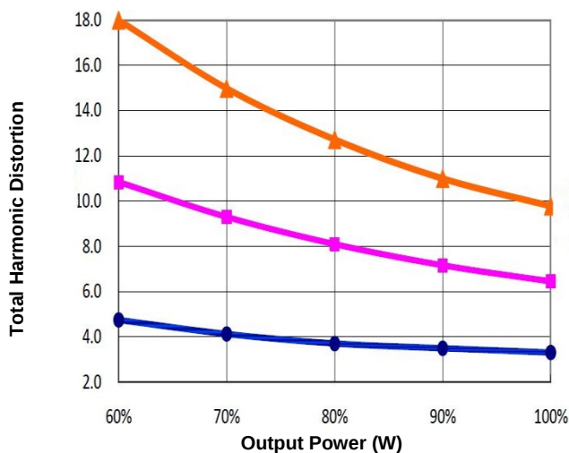
Figure 12: Total Harmonic Distortion vs. Output Power
