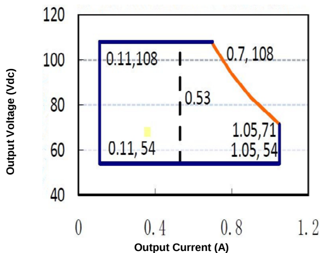
Figure 3: Typical V-I Characteristic Curve (LUB075X-108C)
