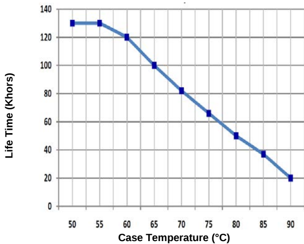
Figure 10: Life Time vs. Case Temperature
