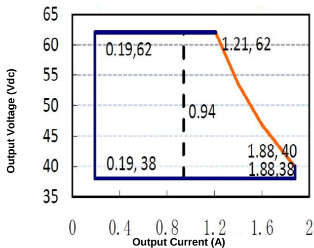
Figure 2: Typical V-I Characteristic Curve (LUB075X-062C)
