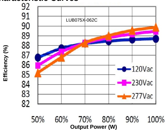
Figure 4: Efficiency vs. Output Power ( I_o=1.21A )
